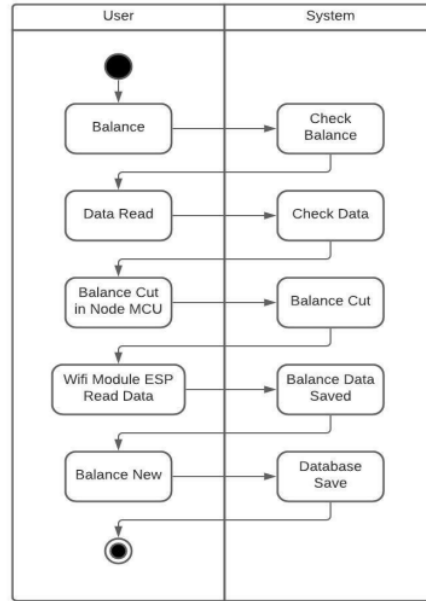
Fig. 4. Activity diagram
