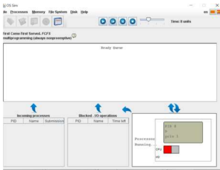
FIGURE 12. STEP BY STEP SIMULATION IMPLEMENTATION AT T=7
