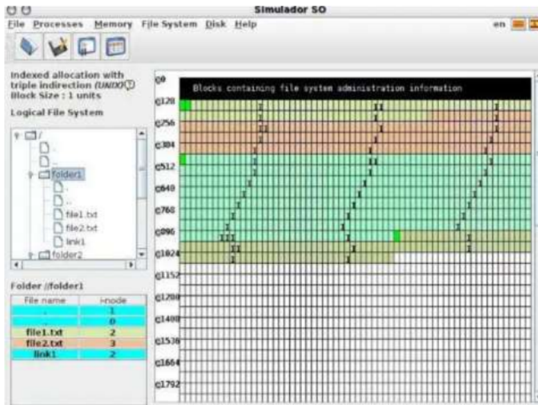
FIGURE 5. FILE MANAGEMENT
