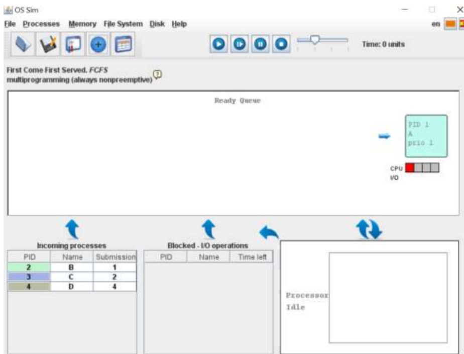
FIGURE 6. SIMULATION IMPLEMENTATION OF TABLE 1.
