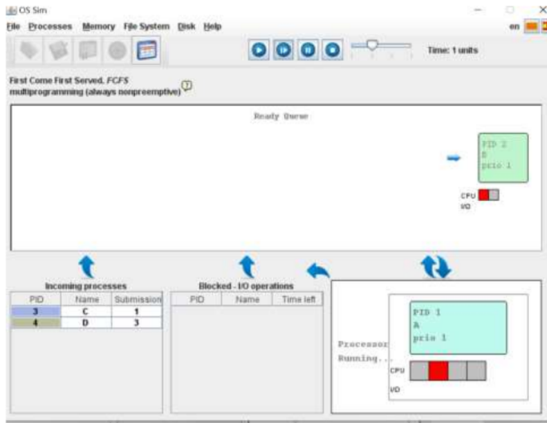
FIGURE 7. STEP BY STEP SIMULATION IMPLEMENTATION AT T=2
