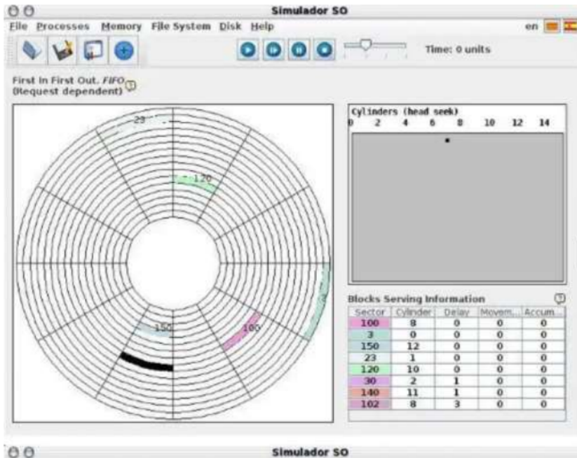
FIGURE 4. DISK ALLOCATION IN SECTORS, TRACKS, AND CLUSTER.
