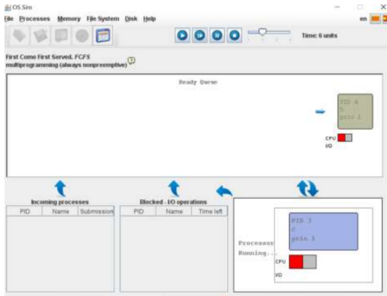
FIGURE 11. STEP BY STEP SIMULATION IMPLEMENTATION AT T = 6
