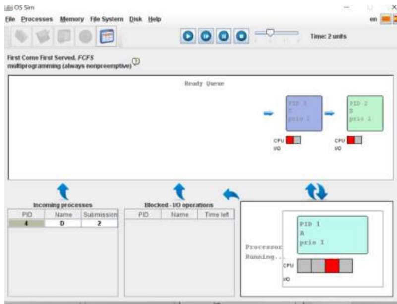
FIGURE 8. STEP BY STEP SIMULATION IMPLEMENTATION AT T=3
