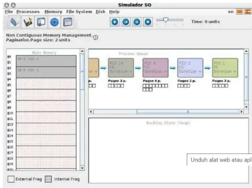
FIGURE 3. MEMORY MANAGEMENT
