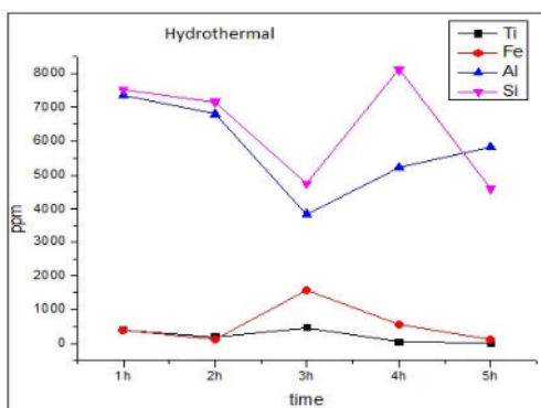
FIGURE 3. ICP-OS results of the filtrate after hydrothermal process
