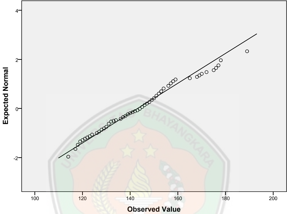
Normal Q-Q Plot of SWB
