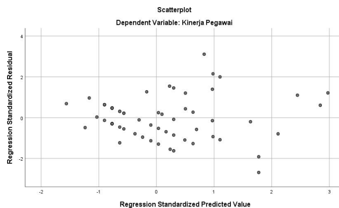
Figure 1. Heteroscedasticity Test
