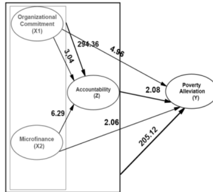
Figure 3 Calculation Results Structural Equation Model (t-value model)
