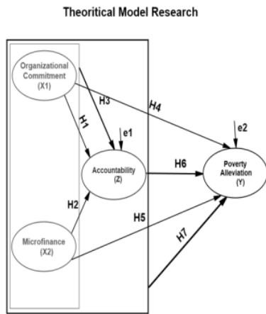
Figure 1. Theoretical Model Research
