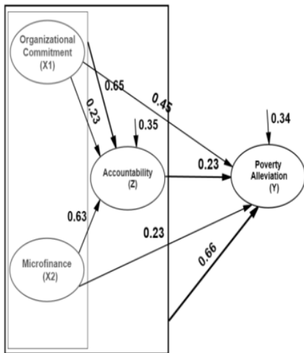
Figure 2 Calculation Results Structural Equation Model (Standardized Model)
