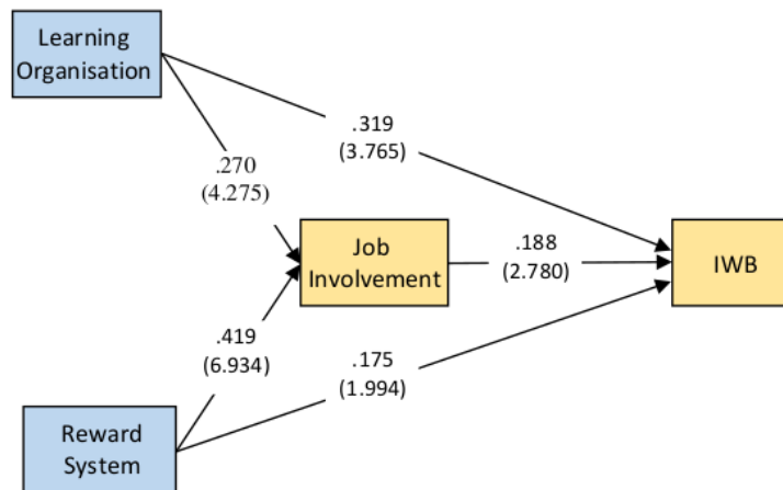
Figure 1. Path coefficients and t values
