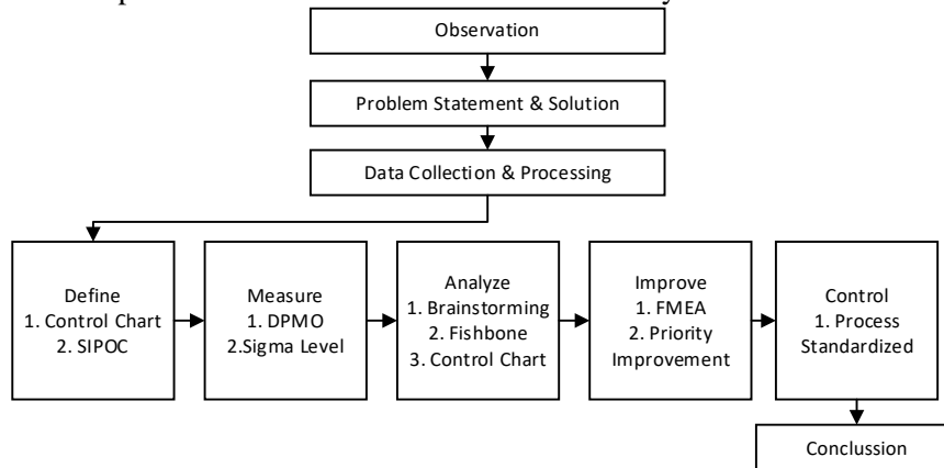
Figure 1. Research Framework
