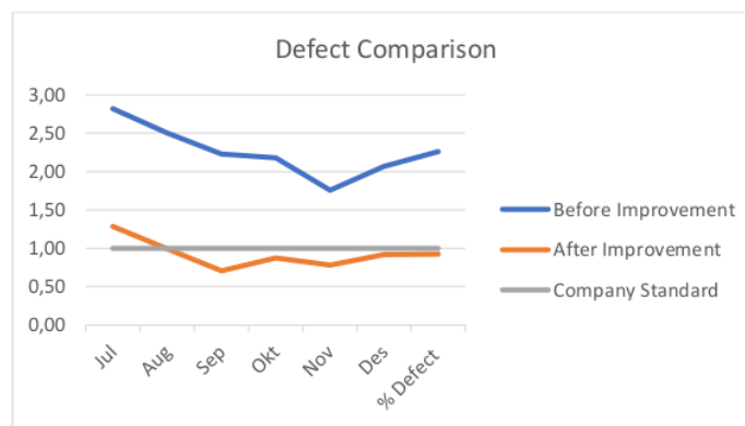
Figure 6. Defect comparison.
