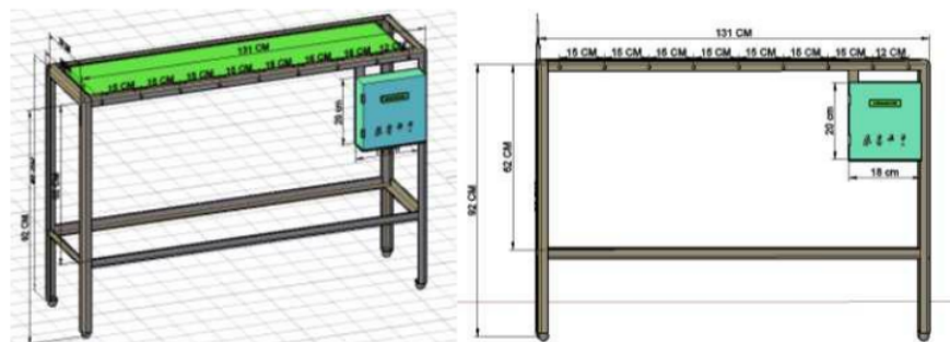
Figure 4. Conveyor table design.
