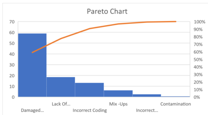
Figure 3. Pareto Diagram
