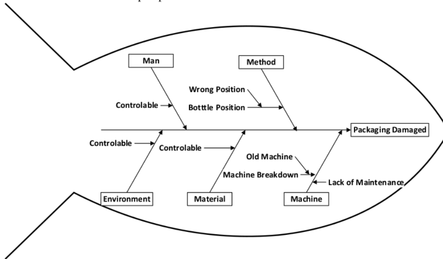
Figure 5. Fishbone Diagram
