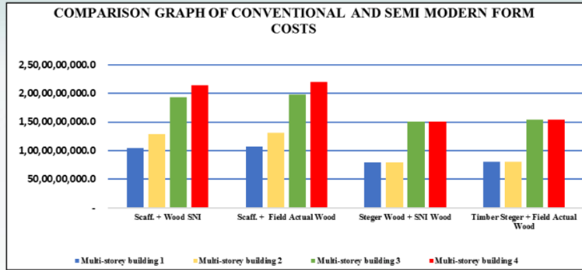
Figure 1 Overall Formwork Cost Comparison
