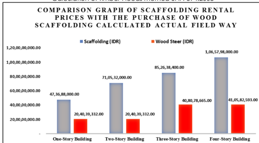
Figure 3 Comparison of Scaffolding Rental Prices with the Purchase of Wooden Stagers Calculation of Timber Needs Actual Field Method
