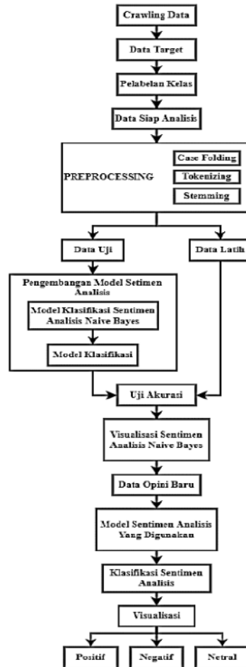
Gambar 1. Model Analisis Sentimen
