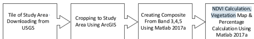
Fig. 2 Research Framework
