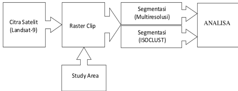
Fig. 2 Segmentation Process
