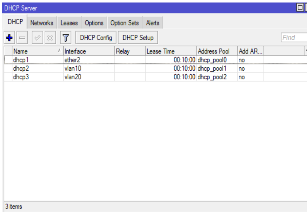
Gambar 5. DHCP
