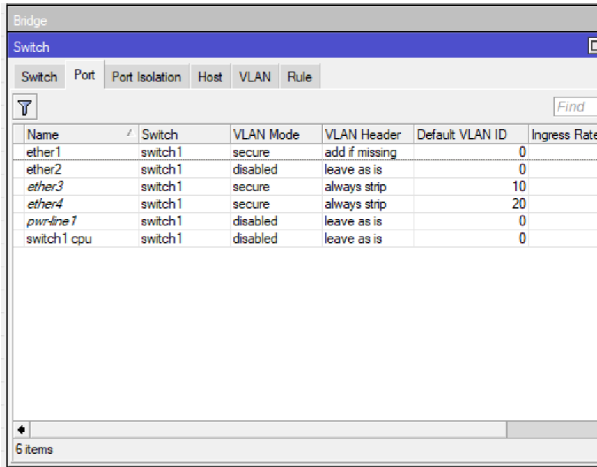
Gambar 8. Port Bridge
