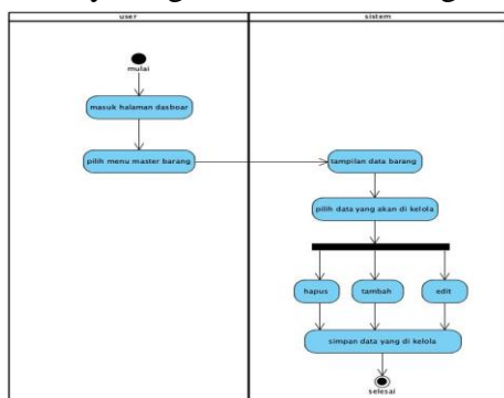
Gambar 4.5 Activity Diagram Master Barang
