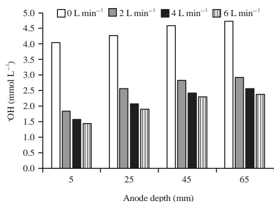
Fig. 4: Amount of ·OH generated at temperature 55 °C
