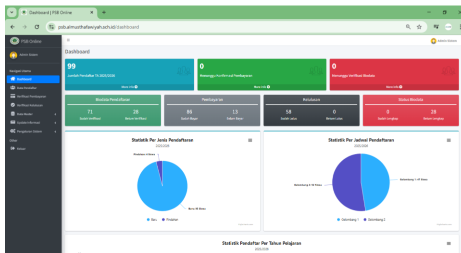
Gambar 2. Dashboar Administrator
