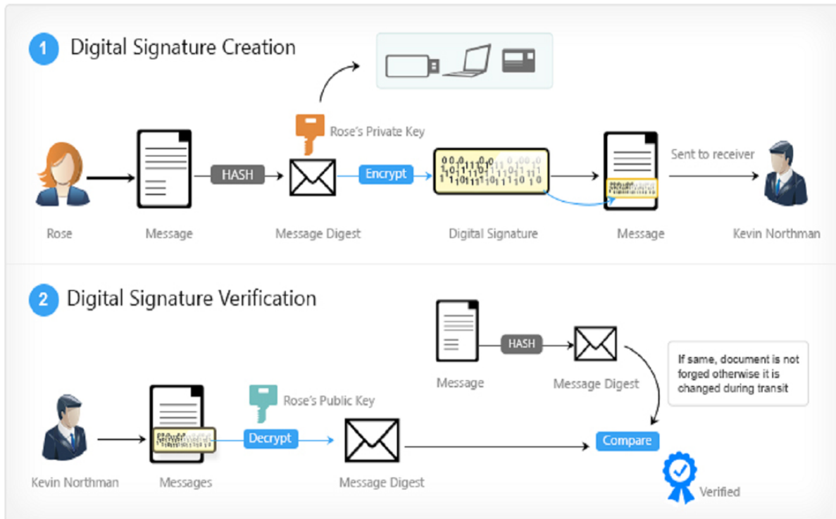
FIGURE 1. Process for creating and verifying electronic signatures [10]
