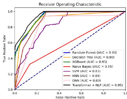
Figure 4. ROC for 80-20 Model
