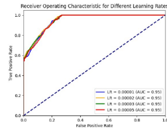
Figure 5. ROC Curve for Sensitivity Analysis of Parameters
