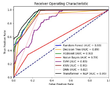
Figure 4. ROC for 80-20 Model
