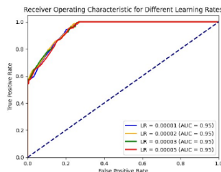
Figure 6. ROC Curve for Sensitivity Analysis of Parameters
