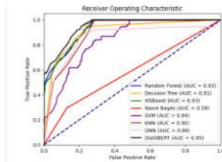
Figure 2. ROC for 90-10 Model
