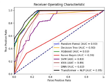
Figure 4. ROC for the 70-30 Model
