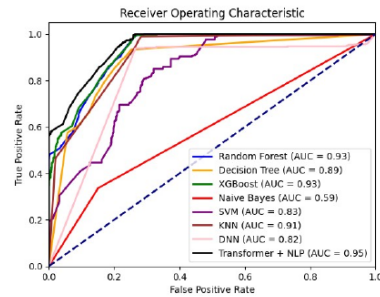
Figure 3. ROC for 80-20 Model
