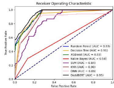
Figure 2. ROC for 90-10 Model
