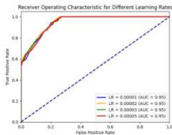
Figure 5. ROC Curve for Sensitivity Analysis of Parameters
