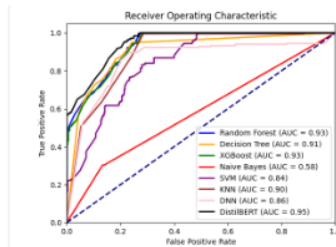
Figure 2. ROC for 90-10 Model
