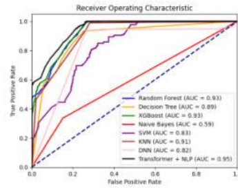
Figure 3. ROC for 80-20 Model
