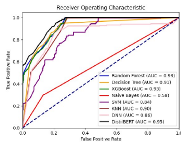
Figure 3. ROC for 90-10 Model
