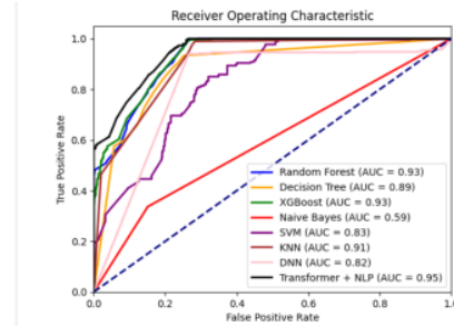
Figure 3. ROC for 80-20 Model
