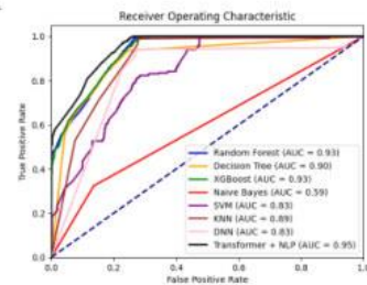
Figure 4. ROC for the 70-30 Model
