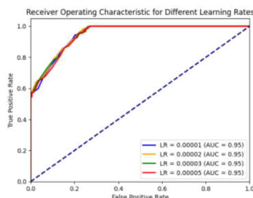
Figure 5. ROC Curve for Sensitivity Analysis of Parameters
