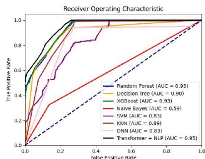
Figure 4. ROC for the 70-30 Model
